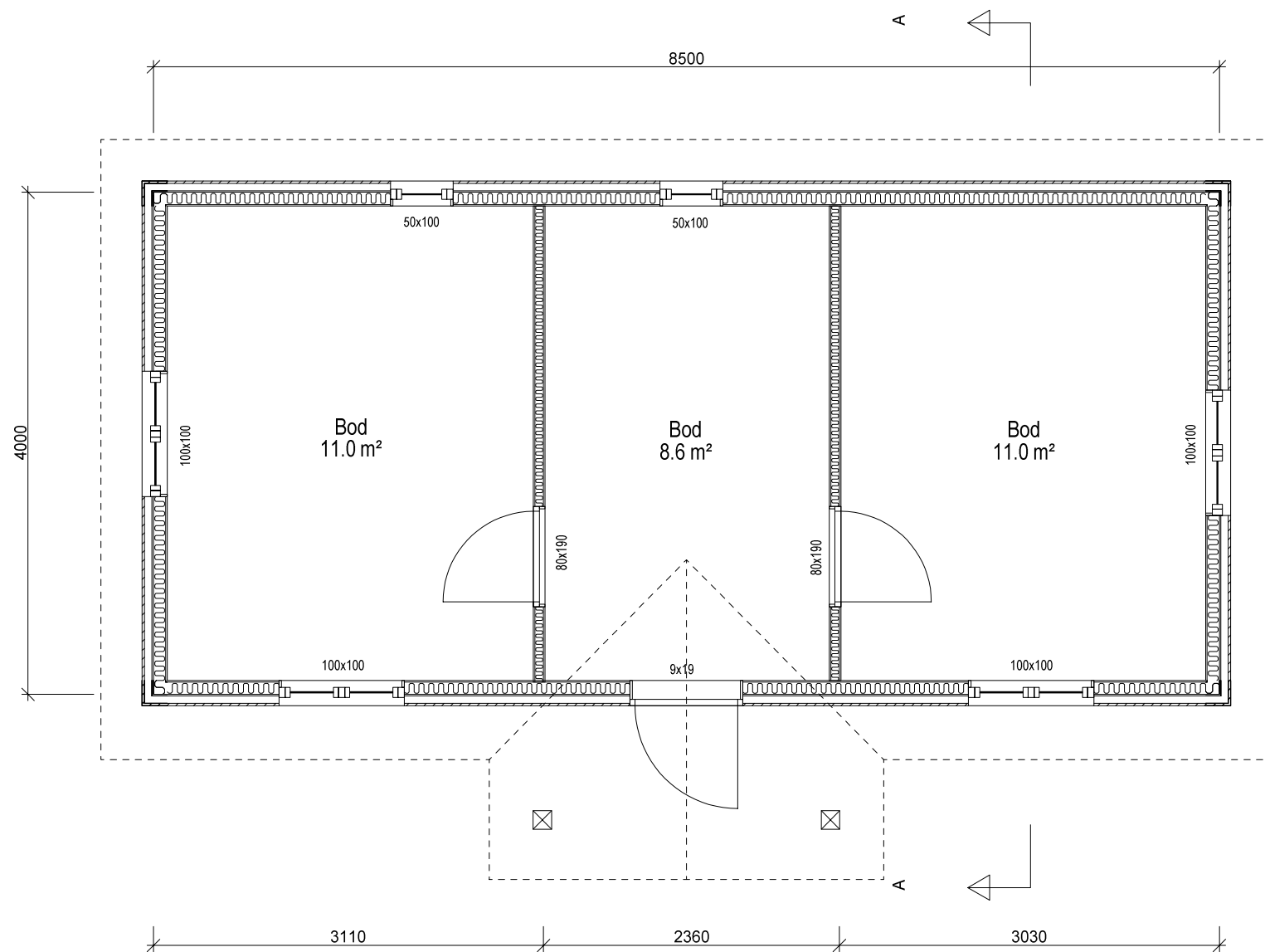
Plan
